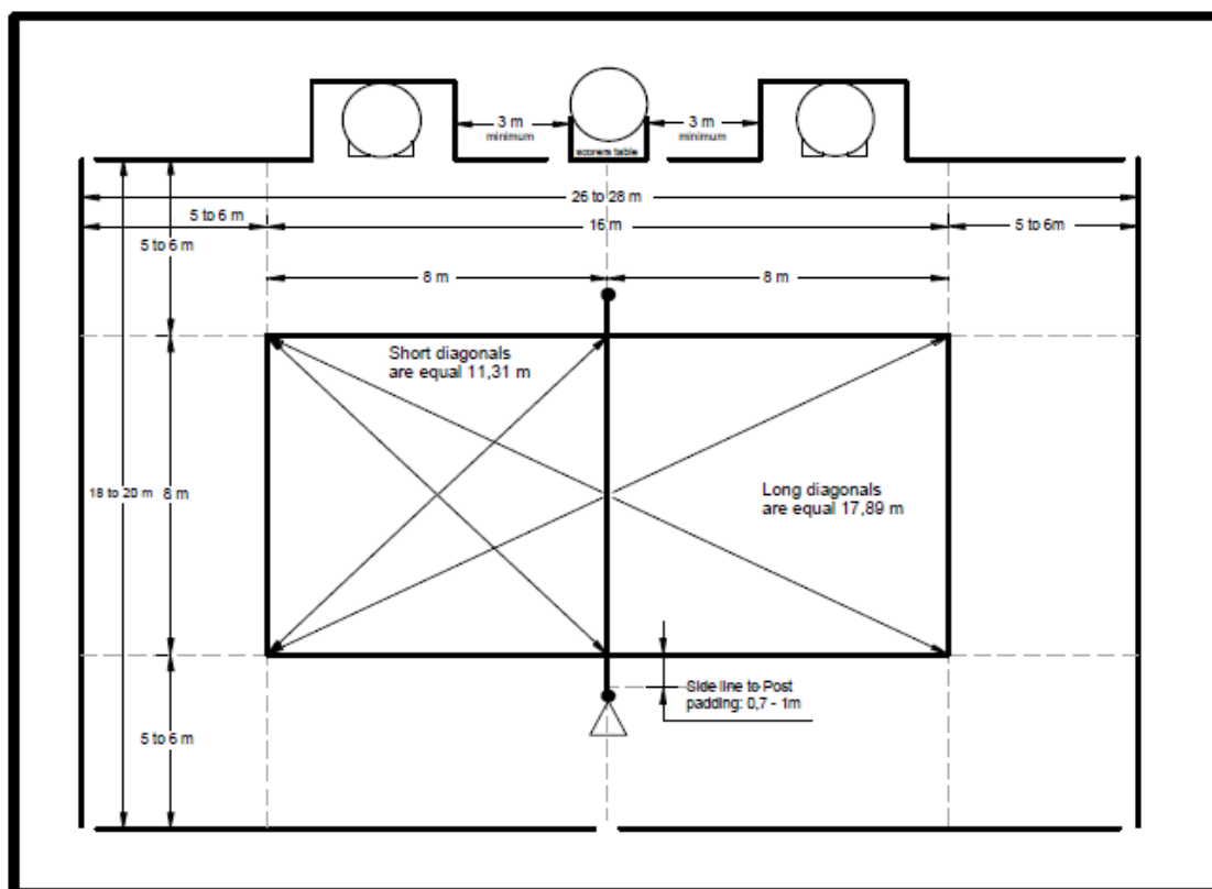
Figure 1 - veld layout
